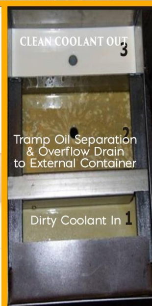
OSP-TOS2054-P Portable 250-1000 Gallons
