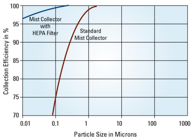
Particle Size vs. Collection Efficiency
