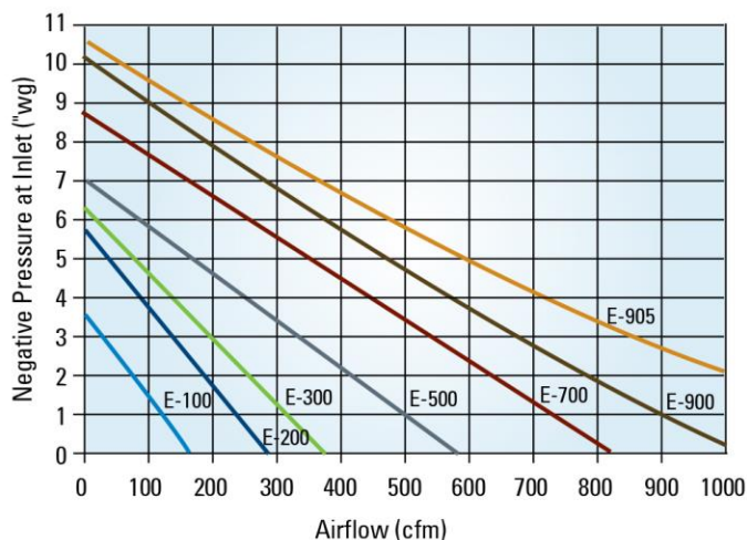
Airflow at 60 Hz - 3450 RPM
