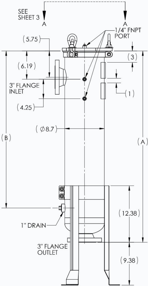
REFERENCE ENGINEERING DRAWING 21136
