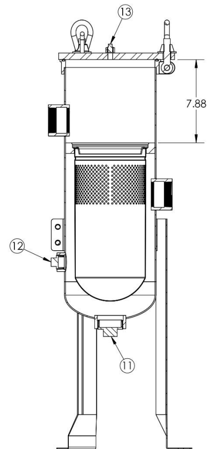
SECTION B-B
