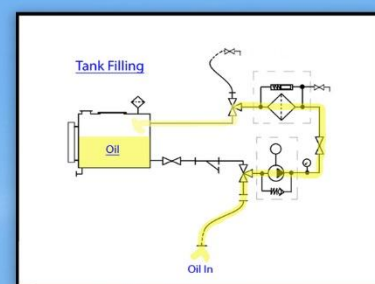
Oil Tank Fill and Oil Storage
