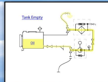
Oil Tank Transfer Out and Filter
